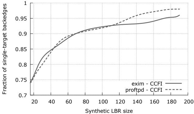
Figure 3: Fraction of single-target backedges for CCFI (two applications with most sensitive calls) when simulating an increasingly large LBR.
